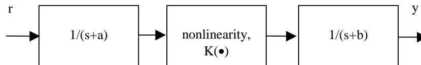
Figure 1 Structure of nonlinear system in Example 3
