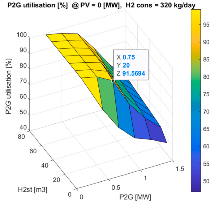
Fig. 19. Hydrogen-system utilisation rate in November.
