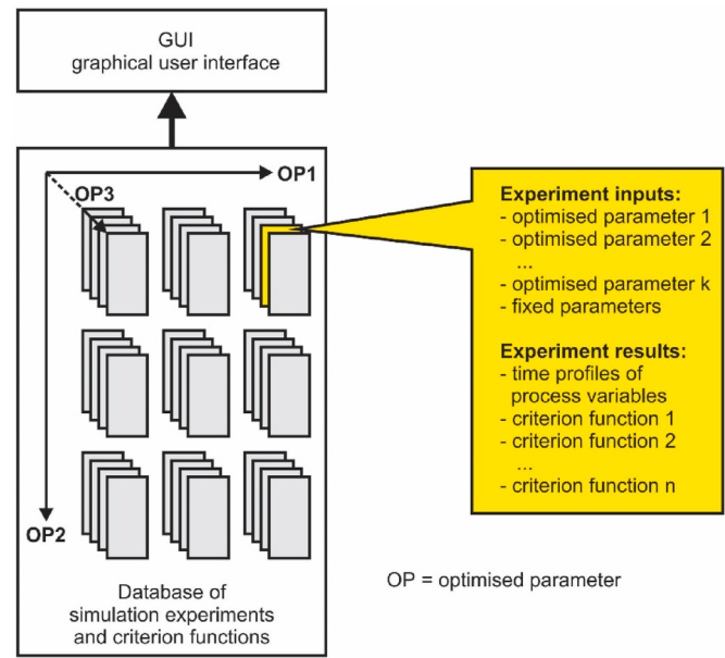
Fig. 3. Hydrogen-system-configuration explorer.
