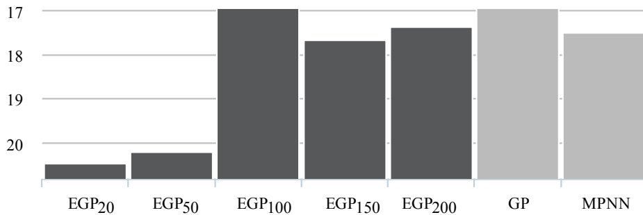
Figure 2. Root mean squared error – RMSE measure for EGP models with various active set sizes compared to full GP model and MPNN model, both trained by using full training set of 488 samples.
