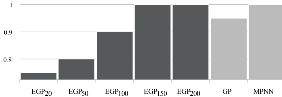
Figure 4. Performance index – p^6 measure for EGP models with various active set sizes compared to full GP model and MPNN model, both trained by using full training set of 488 samples.
