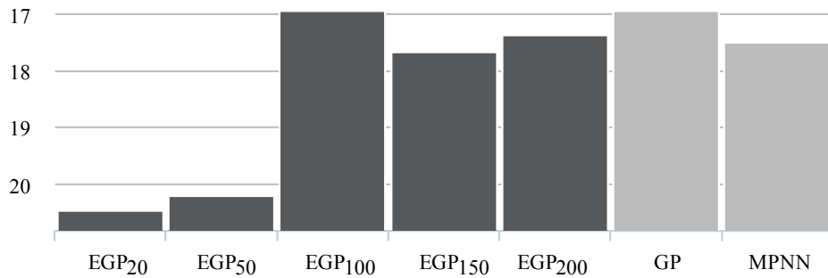
Figure 3. Success index – SI measure for EGP models with various active set sizes compared to full GP model and MPNN model, both trained by using full training set of 488 samples.
