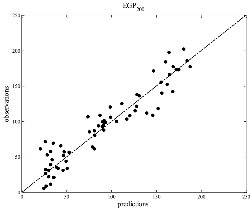
Figure 6. Scatter plot of errors between predictions of the maximal ozone concentration (one day ahead) and observations for validation data set.
