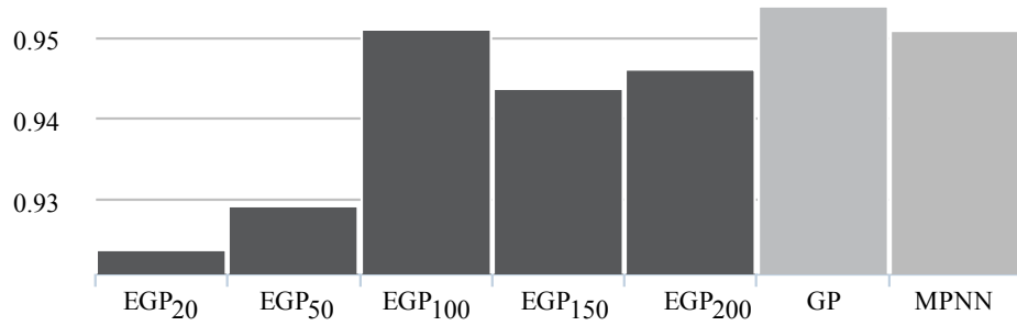
Figure 1. Correlation factor – CF measure for EGP models with various active set sizes compared to full GP model and MPNN model, both trained by using full training set of 488 samples.
